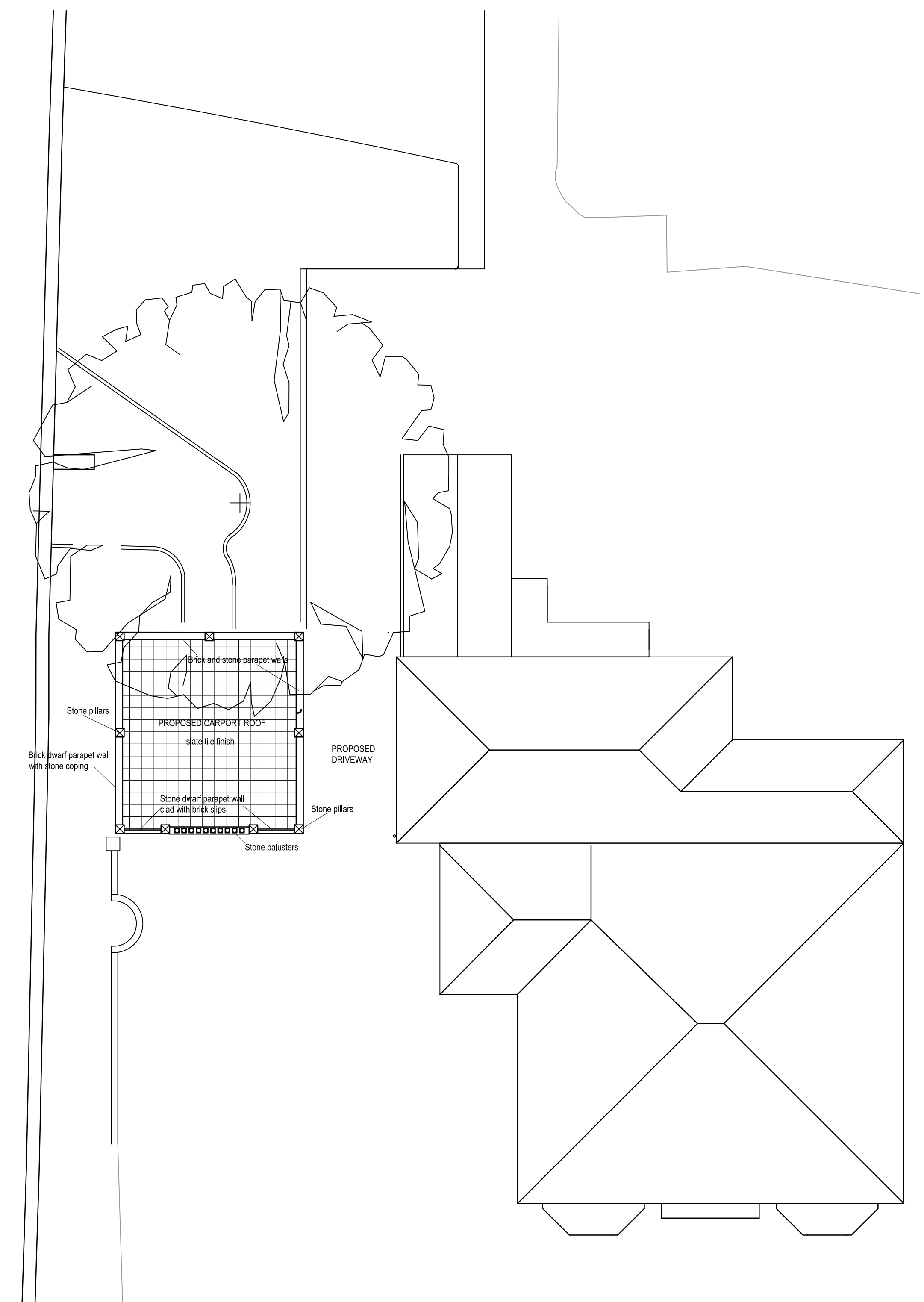
PROPOSED SITE LAYOUT PLAN AT ROOF LEVEL- Scale 1:100
